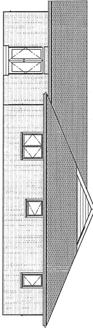
EAST ELEVATION
